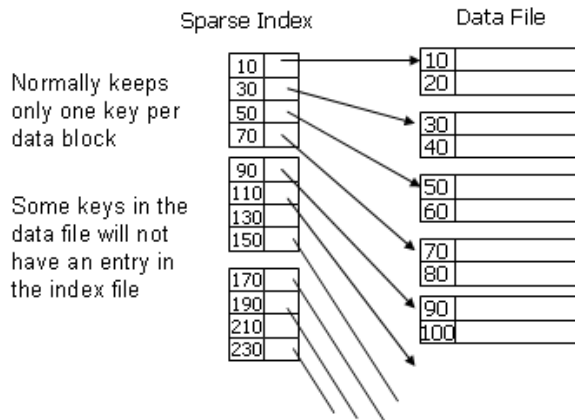
Figure-26.2: Sparse index concept
