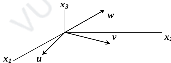
Linearly independent w not in \text{Span}\{u, v\}
