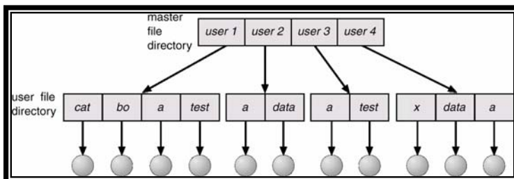
Two-level directory strucutre
