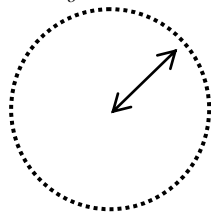
\delta -neighborhood
