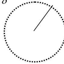
\varepsilon -neighborhood
