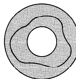
not simply connected
