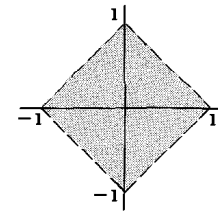
S_{d_2}(p, \delta) is shaded
