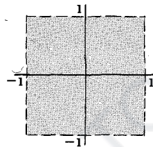
S_{d_1}(p, \delta) is shaded
