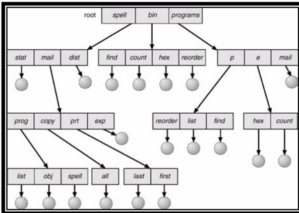
Tree directory structure
