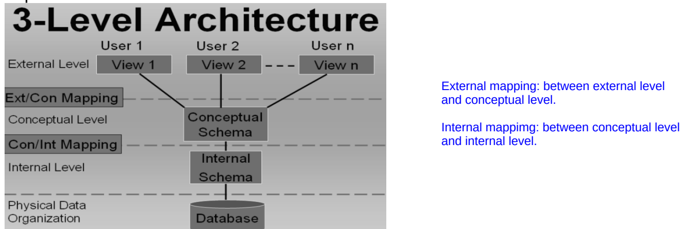
Fig:1: Mapping between External/Conceptual and Conceptual/Internal levels
