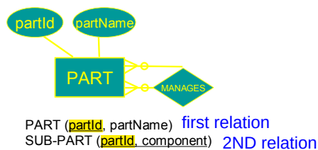
Fig. 4: Recursive many to many relationship and transformation
